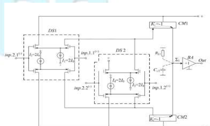
Fig.1.CMOS DDOA functional blocks
